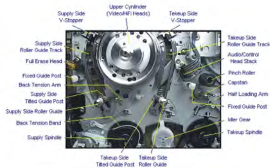
Typical VHS VCR Tape Transport Components
