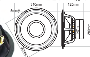
Physical measurements taken from actual stock.
